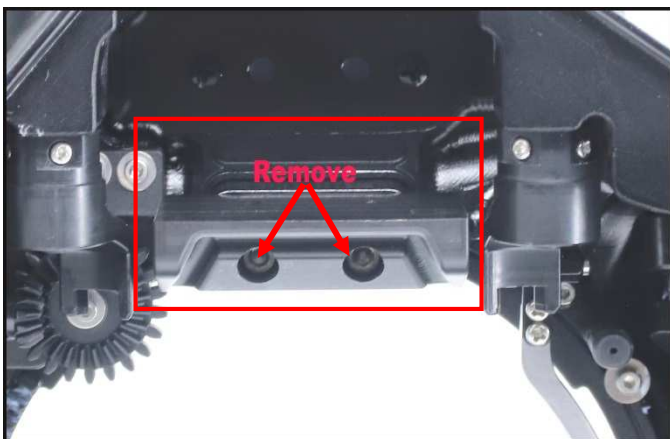
Remove the holder by removing the two screws as indicated above.
